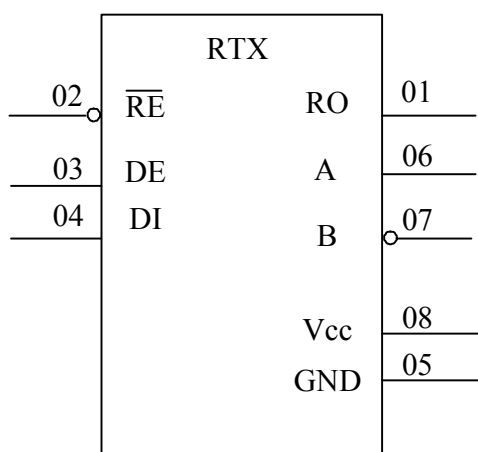
Logic Symbol
