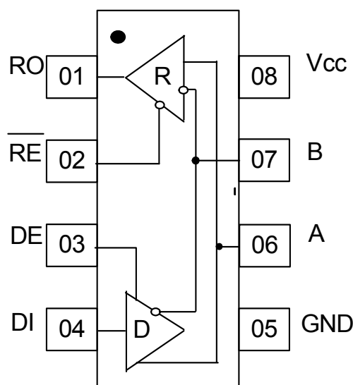
Functional diagram
