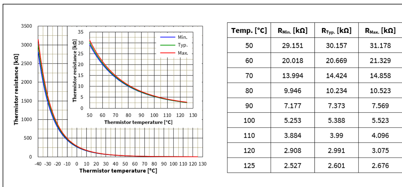
Figure 6 Thermistor resistance – temperature curve and table (For more information, please refer to the application note)
