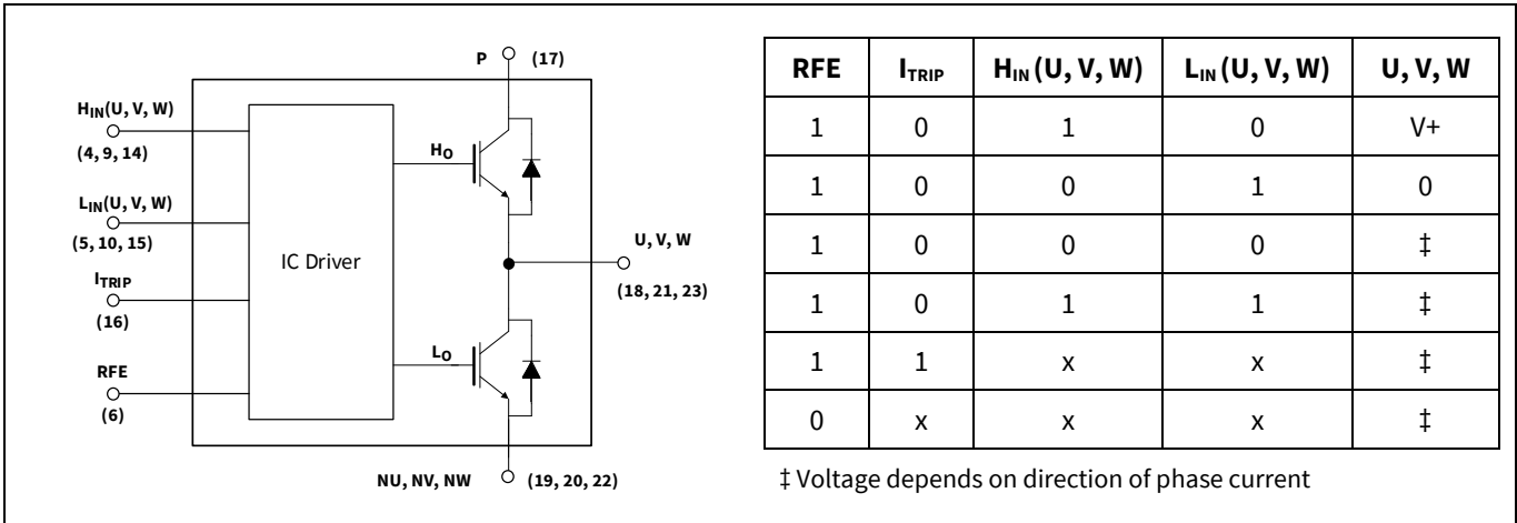
Figure 11 Input-ouput logic table
