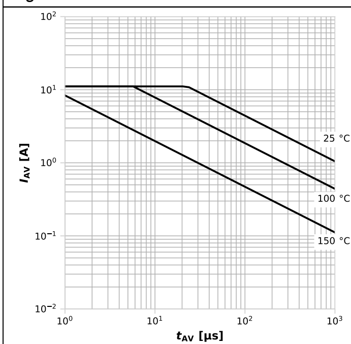
Diagram 19: Avalanche characteristics
