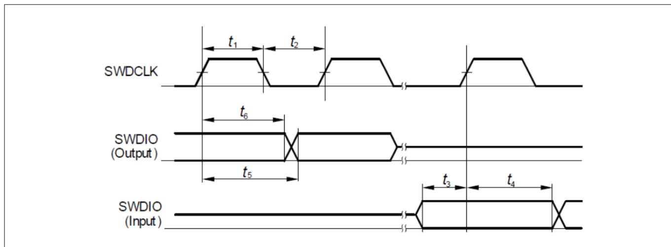
Figure 23 SWD timing
