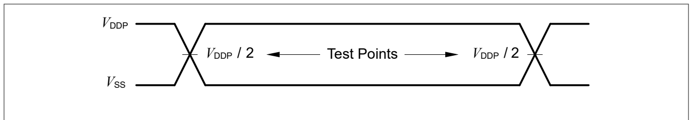
Figure 20 Testing Waveform, Output Delay
