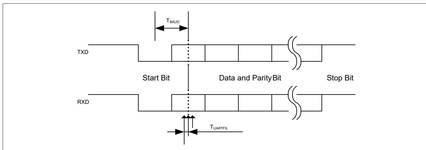
Figure 27 UART timing
