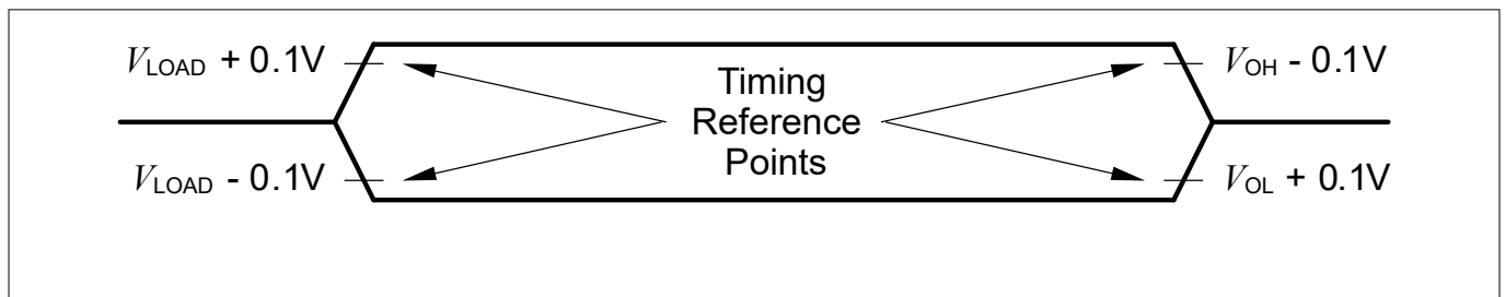
Figure 21 Testing Waveform, Output High Impedance
