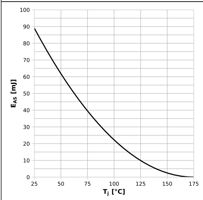
Diagram 13: Avalanche energy
