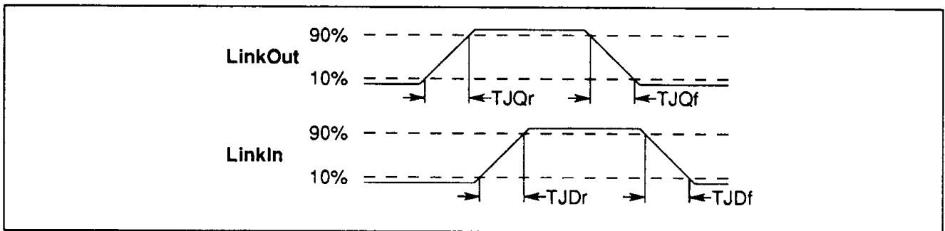
Figure 10.2 IMS T801 link timing
