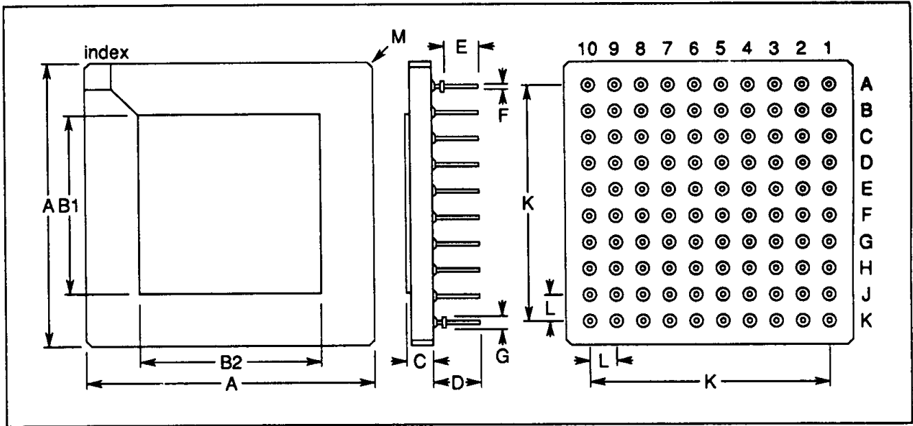
Figure 13.2 100 pin grid array package dimensions
