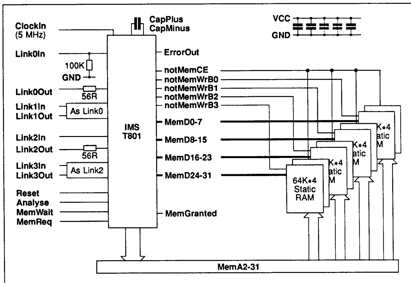
Figure 8.3 IMS T801 static RAM application
