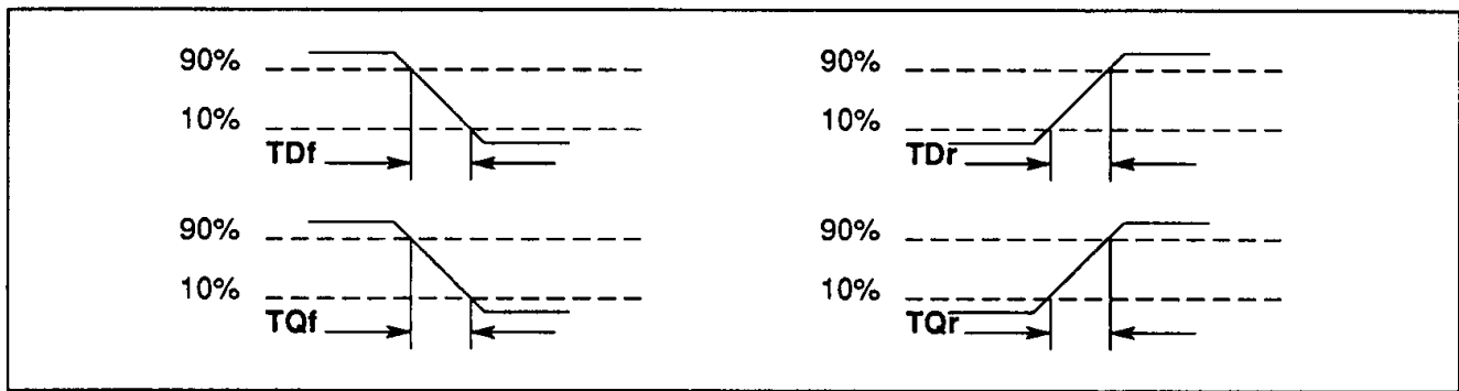
Figure 11.4 IMS T801 input and output edge timing
