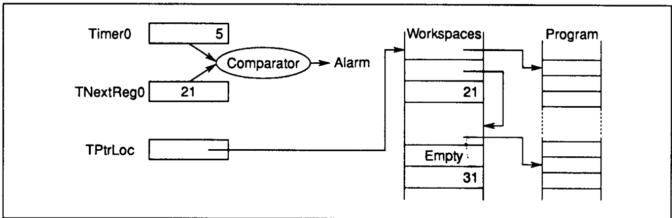
Figure 3.4 Timer registers
