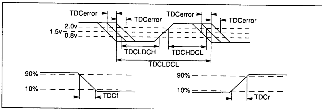
Figure 6.2 ClockIn timing
