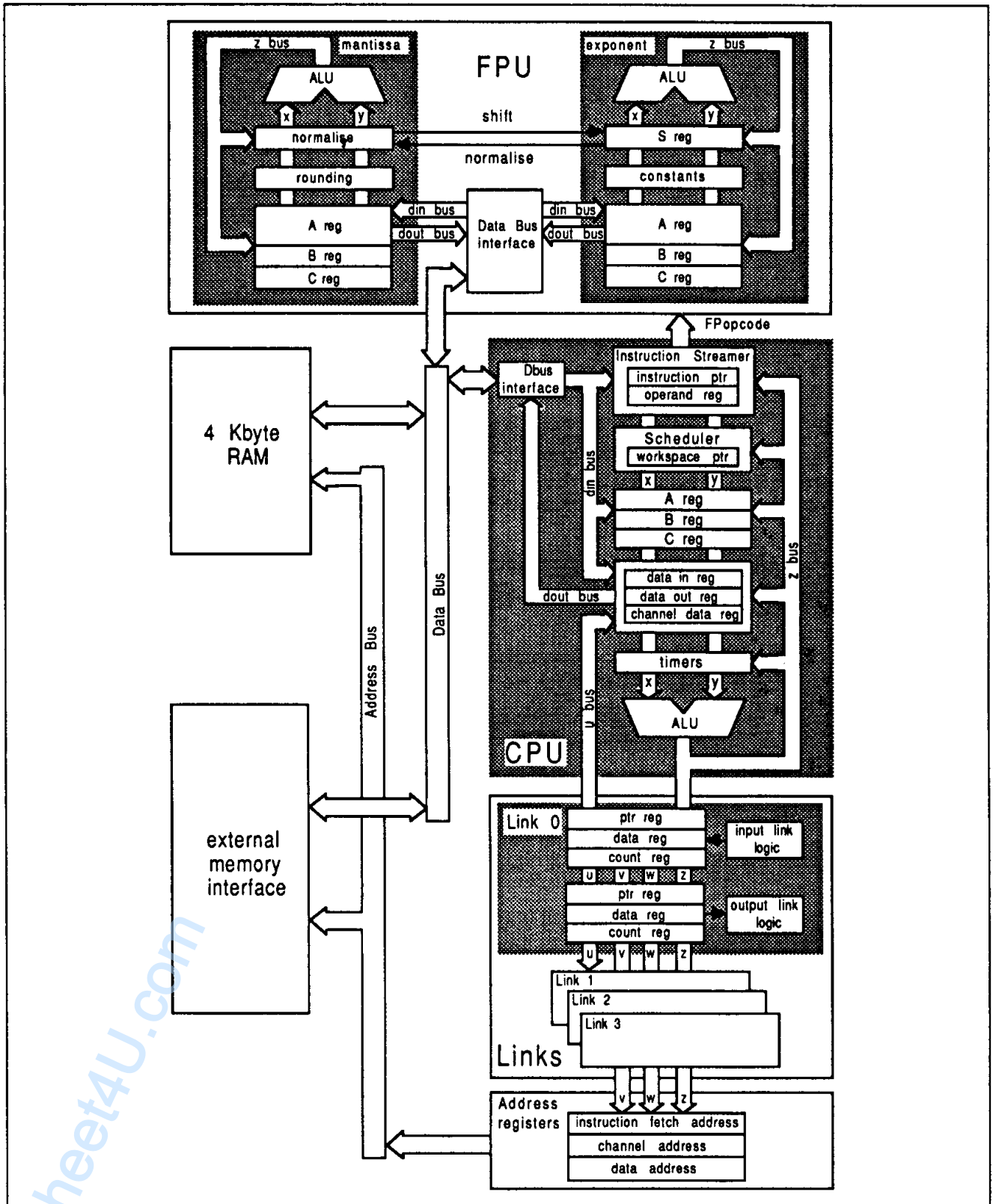
Figure 1.2 IMS T801 internal datapaths
