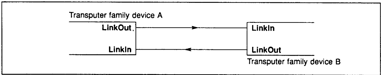
Figure 10.4 IMS T801 Links directly connected
