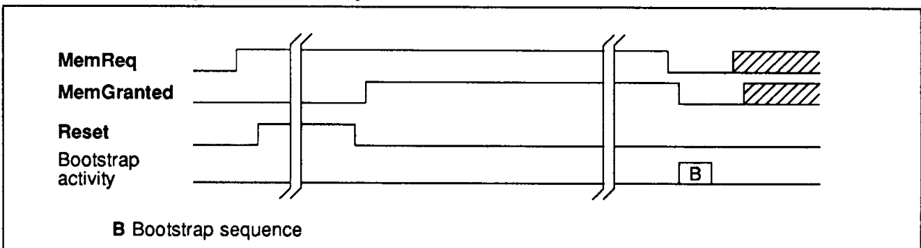
Figure 8.9 IMS T801 DMA sequence at reset
