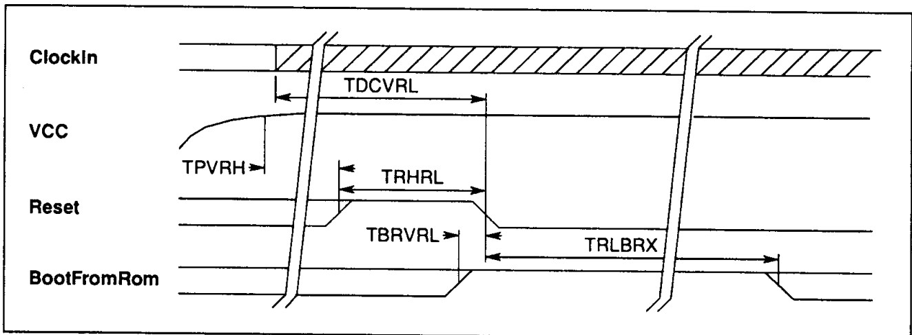
Figure 6.3 Transputer reset timing with Analyse low
