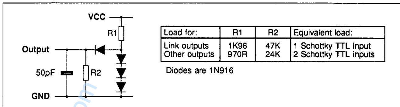
Figure 11.1 Load circuit for AC measurements
