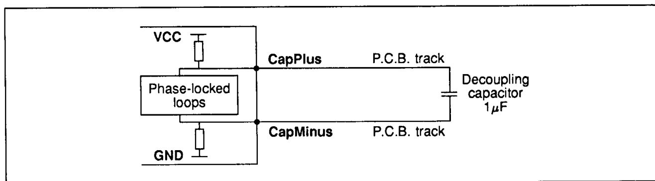
Figure 6.1 Recommended PLL decoupling
