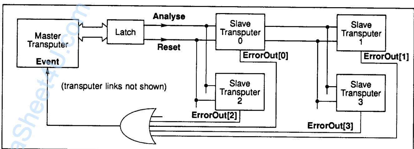
Figure 6.5 Error handling in a multi-transputer system
