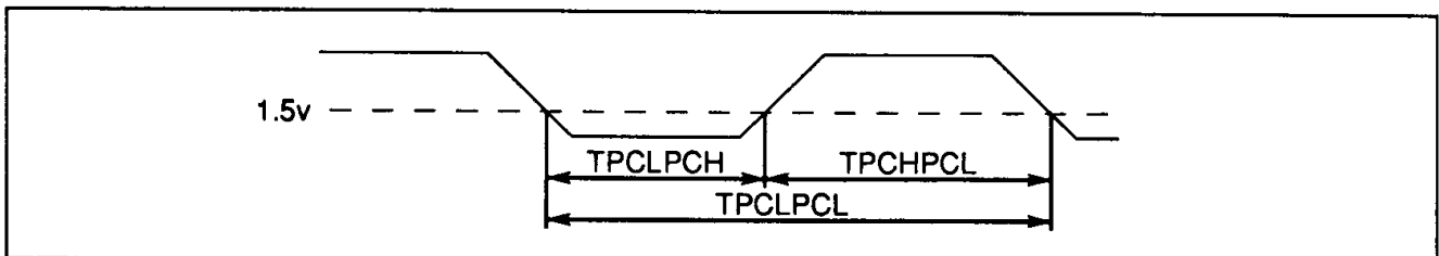
Figure 8.4 IMS T801 ProcClockOut timing
