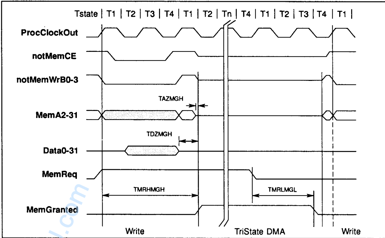
Figure 8.10 IMS T801 memory request timing
