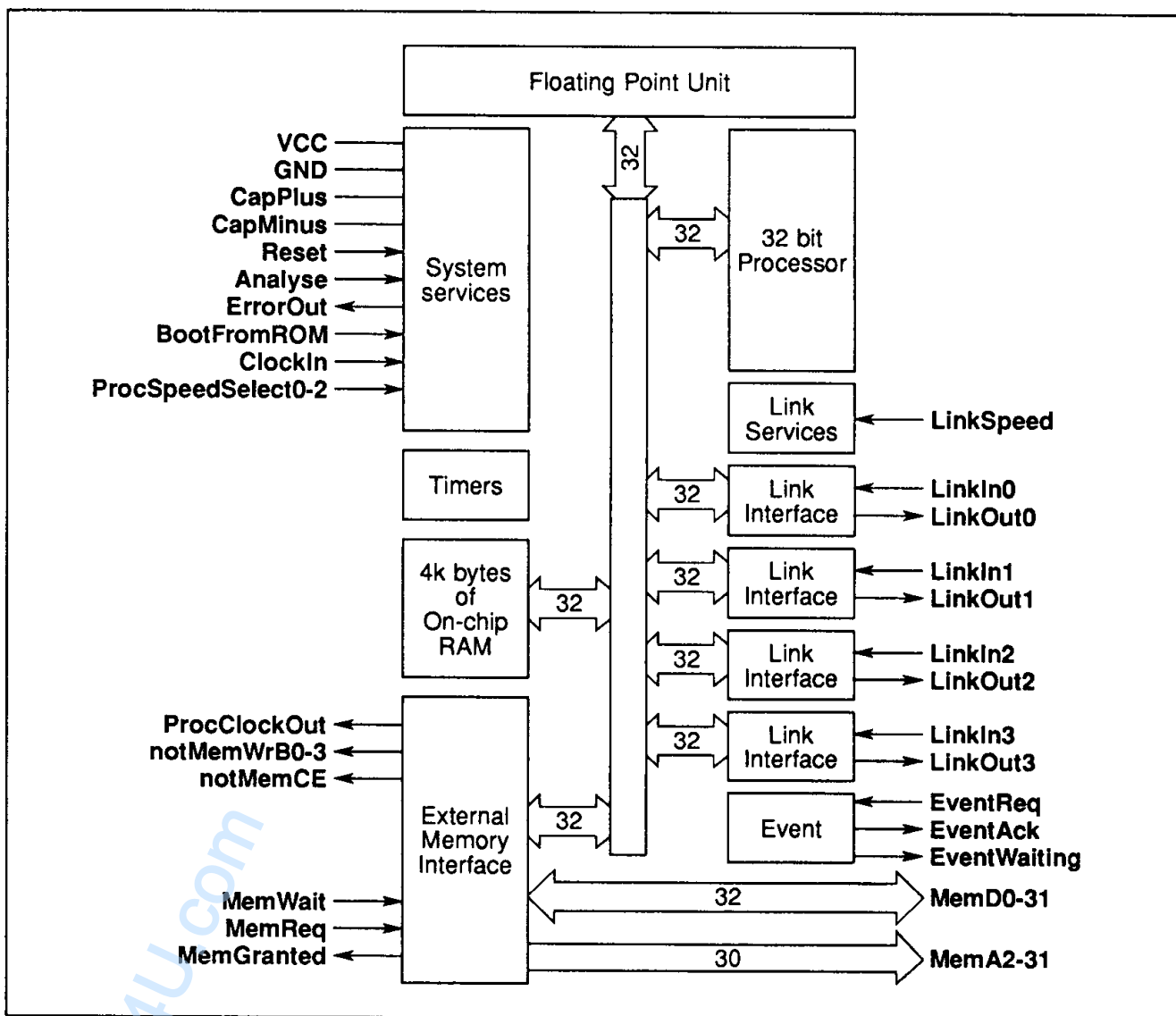
Figure 1.1 IMS T801 block diagram
