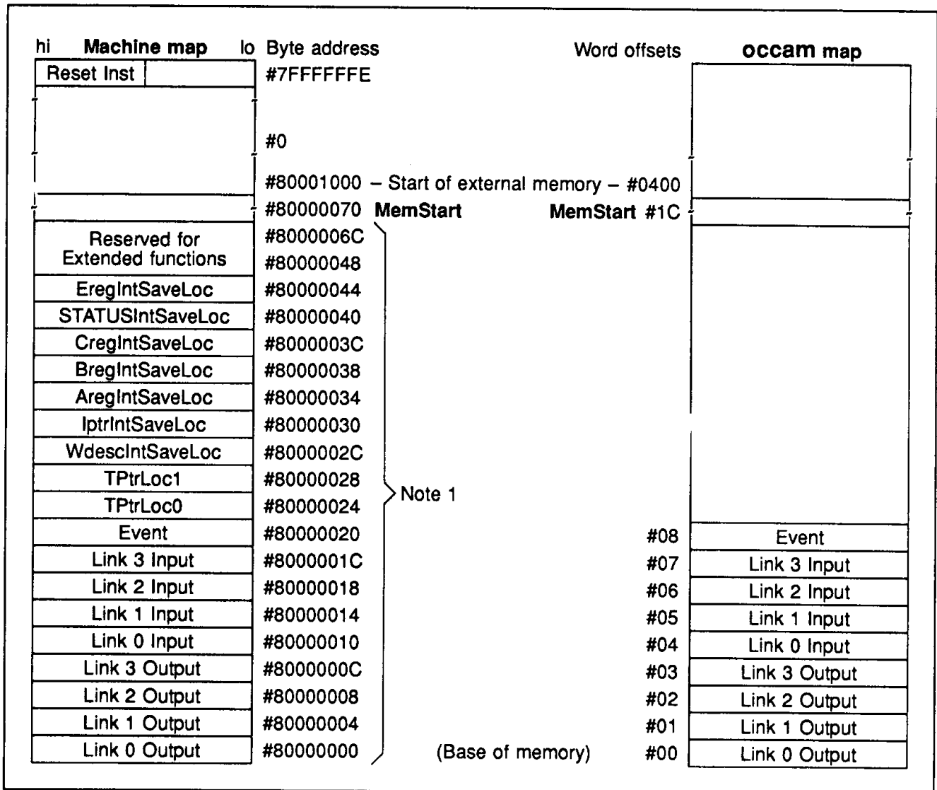
Figure 7.1 IMS T801 memory map
