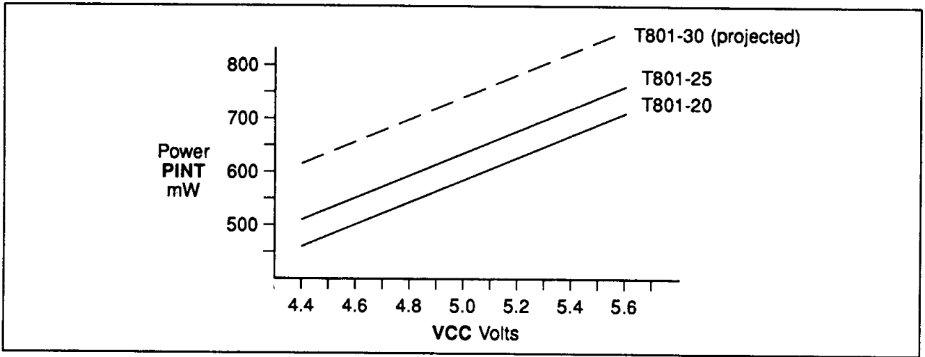
Figure 11.6 IMS T801 internal power dissipation vs VCC
