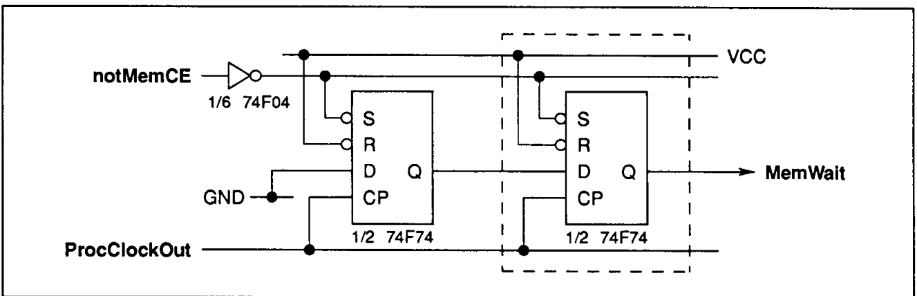
Figure 8.8 Extendable wait state generator
