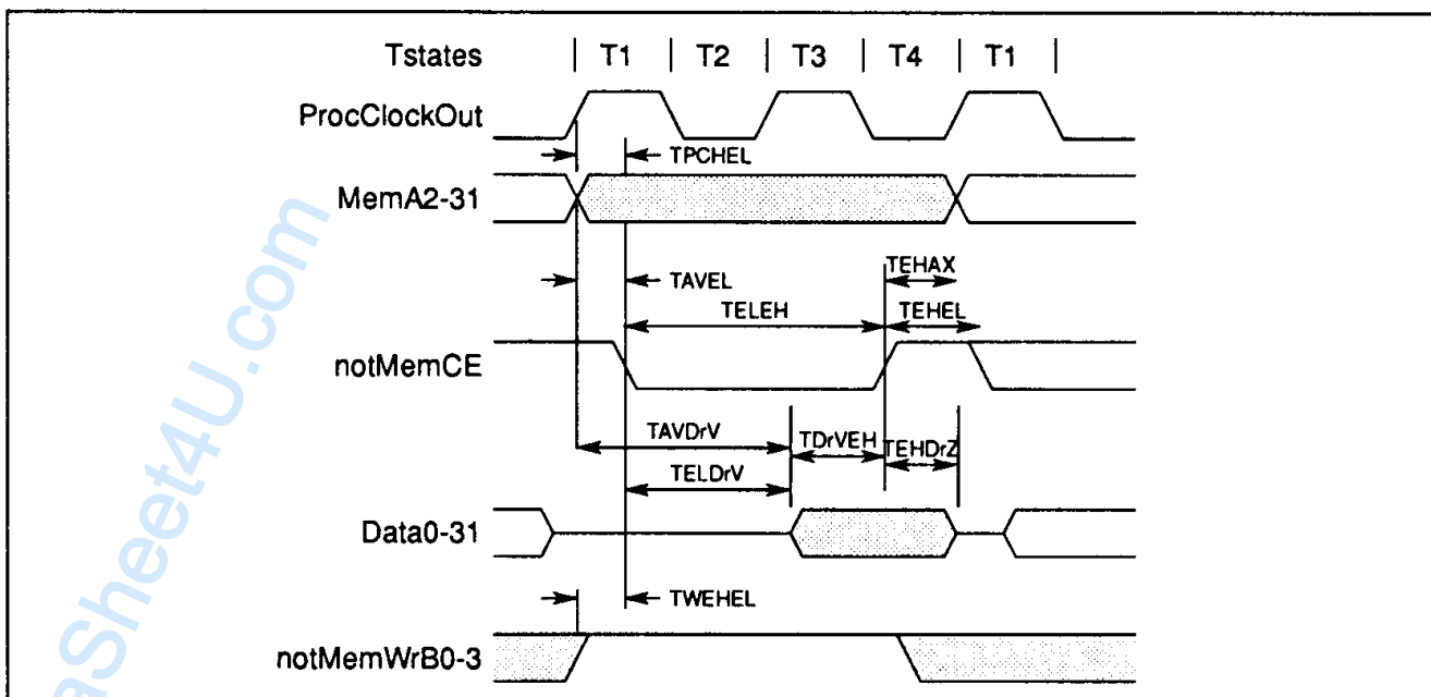
Figure 8.5 IMS T801 external read cycle
