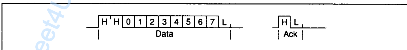
Figure 10.1 IMS T801 link data and acknowledge packets
