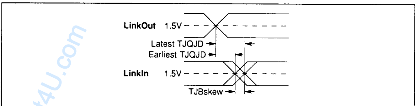
Figure 10.3 IMS T801 buffered link timing
