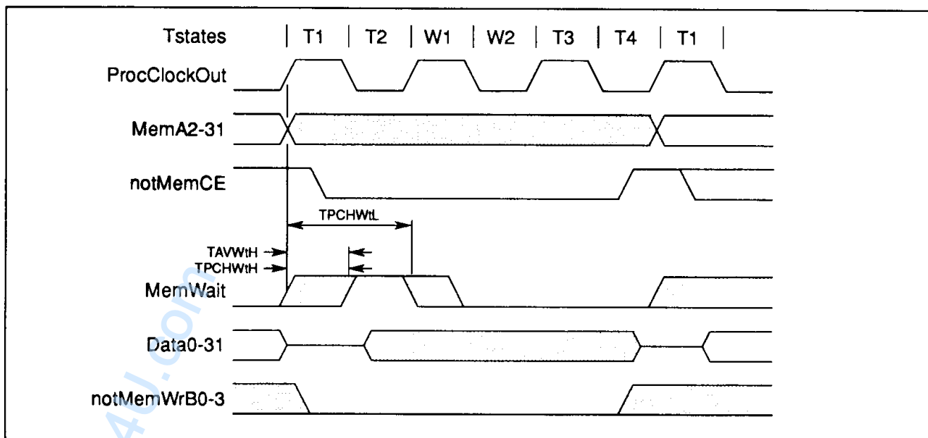
Figure 8.7 IMS T801 memory wait timing
