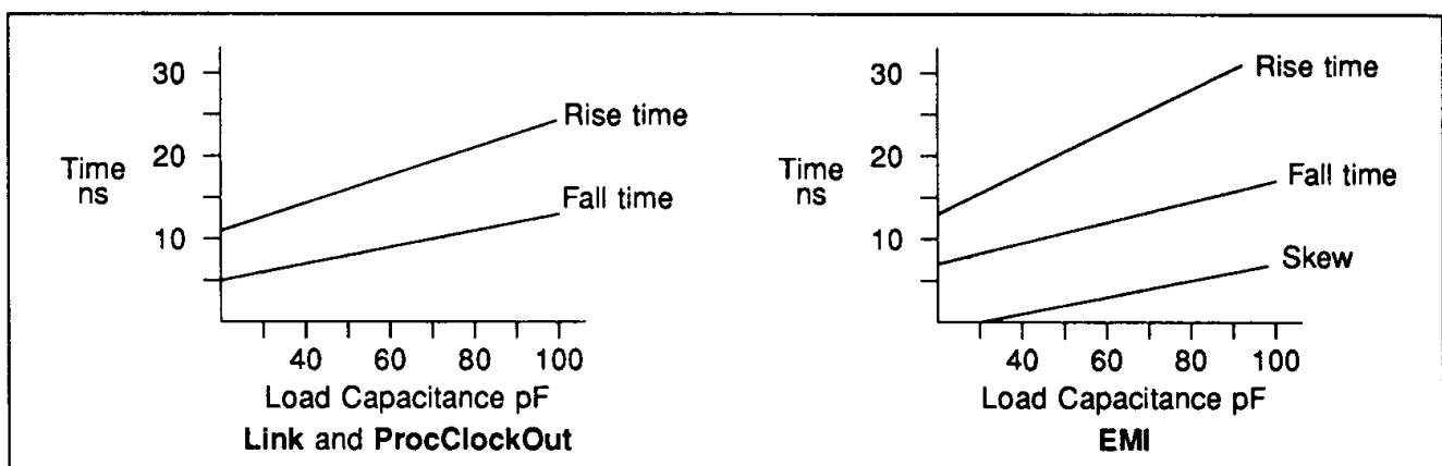
Figure 11.5 Typical rise/fall times
