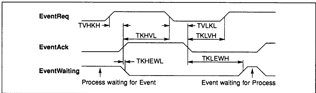
Figure 9.1 IMS T801 event timing
