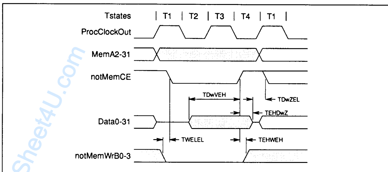
Figure 8.6 IMS T801 external write cycle
