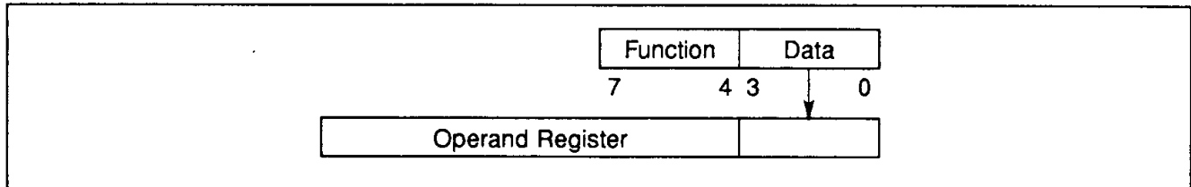
Figure 3.2 Instruction format
