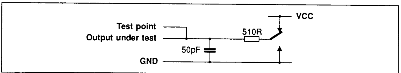
Figure 11.3 Tristate load circuit for AC measurements
