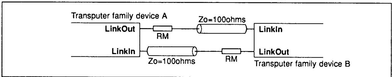
Figure 10.5 IMS T801 Links connected by transmission line
