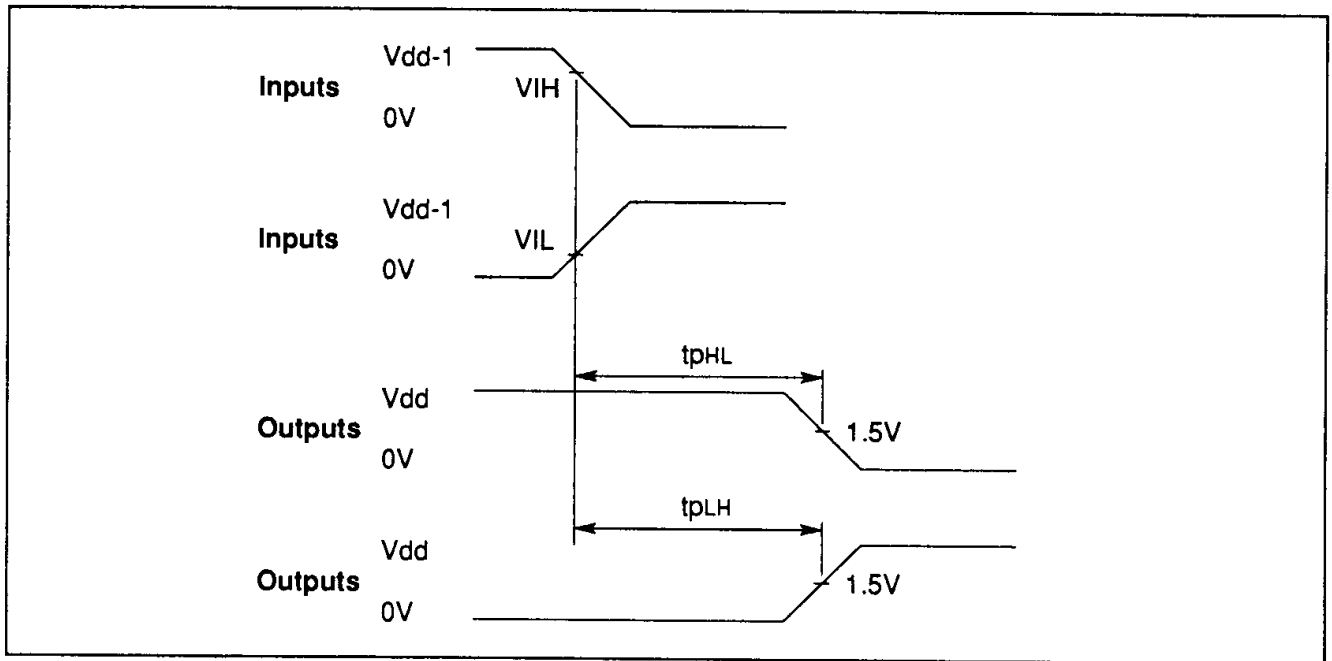
Figure 11.2 AC measurements timing waveforms
