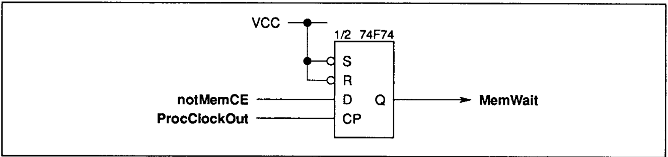
Figure 8.7 Single wait state generator
