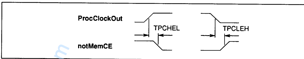
Figure 8.2 IMS T801 skew of notMemCE to ProcClockOut
