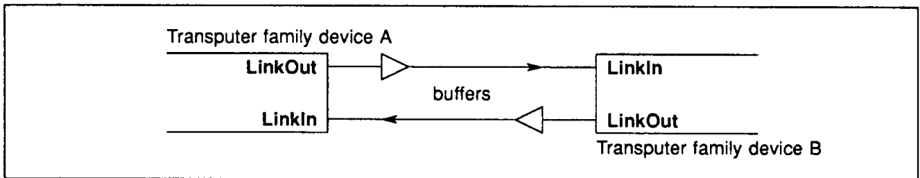
Figure 10.6 IMS T801 Links connected by buffers
