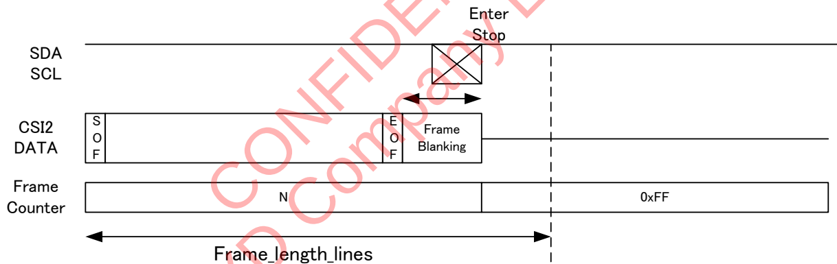
Fig. 22 Software Standby Operation Pattern 2
