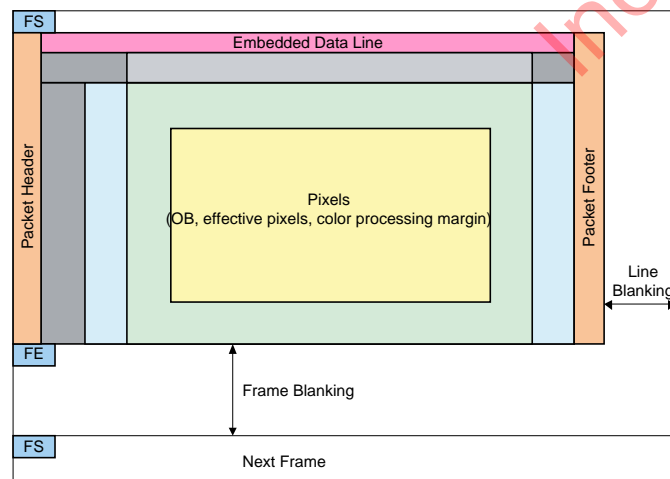
Frame Structure of 4 Lane / 2 Lane
