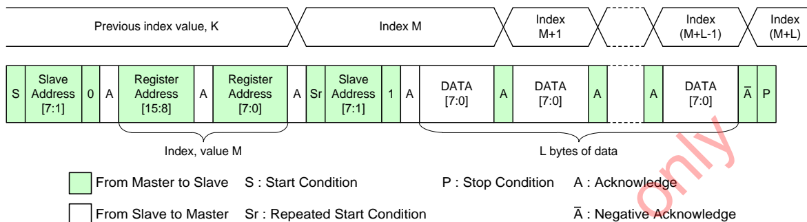
Sequential Read Starting from Random Location
