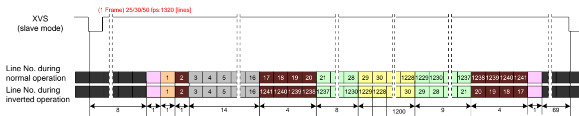
Pixel Array Image Drawing in All-pixel Scan Mode (CSI-2 Serial Output)
