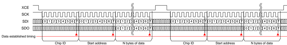
Serial Communication (Discontinuous Addresses)
