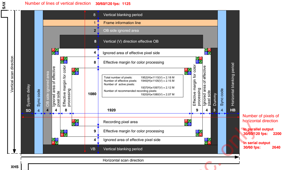
Pixel Array Image Drawing in 1080p-HD Mode
