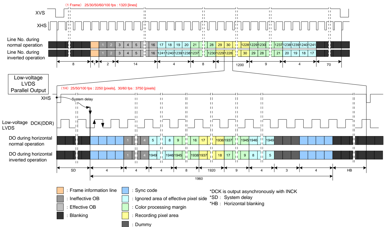
Drive Timing Chart for LVDS Parallel Output in All-pixel Scan Mode
