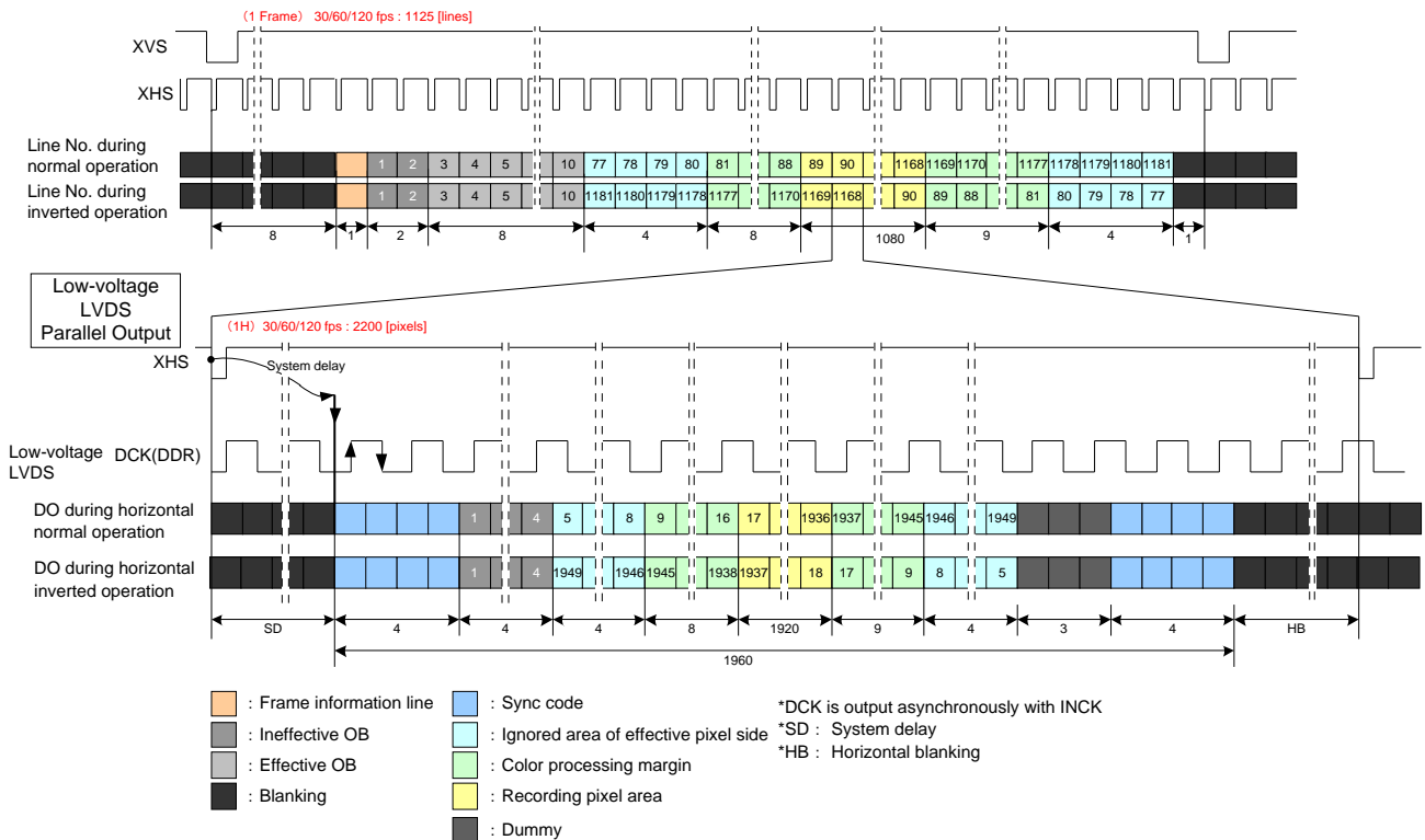
Drive Timing Chart for LVDS Parallel Output in 1080p-HD Mode
