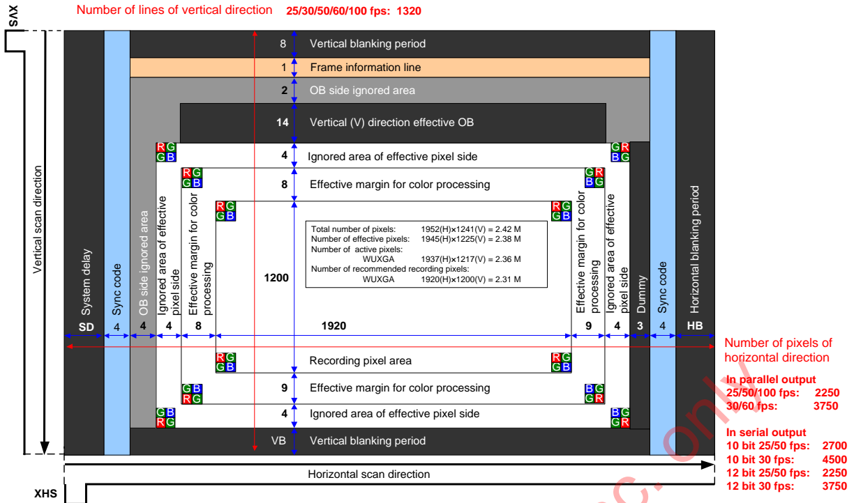
Pixel Array Image Drawing in All-pixel Scan Mode
