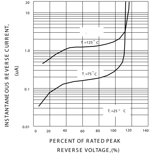
FIG.4-TYPICAL REVERSE CHARACTERISTICS
