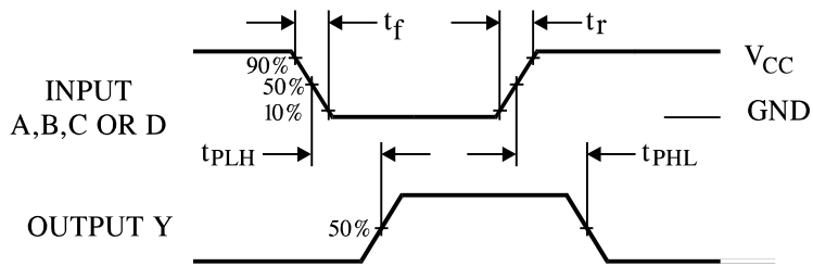
Figure 1. Switching Waveforms
