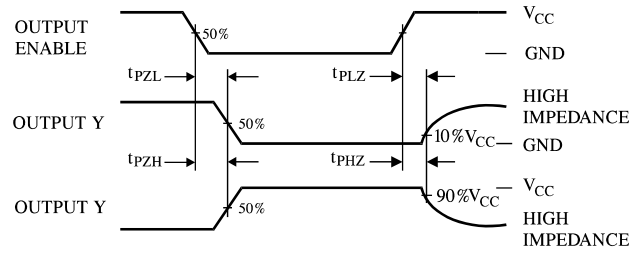
Figure 3. Switching Waveforms
