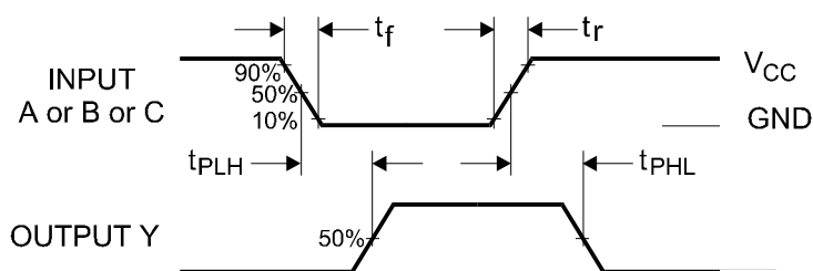
Figure 1. Switching Waveforms
