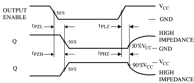
Figure 3. Switching Waveforms
