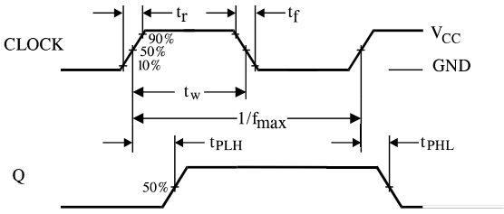
Figure 1. Switching Waveforms
