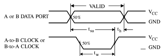
Figure 7. Switching Waveforms
