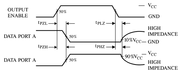
Figure 5. Switching Waveforms
