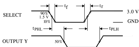
Figure 1. Switching Waveform
