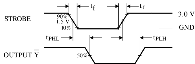
Figure 5. Switching Waveforms
