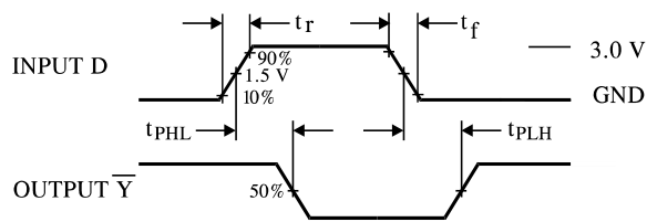
Figure 3. Switching Waveforms
