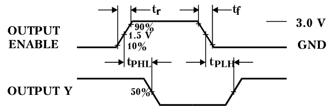
Figure 3. Switching Waveforms
