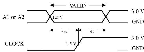
Figure 3. Switching Waveforms
