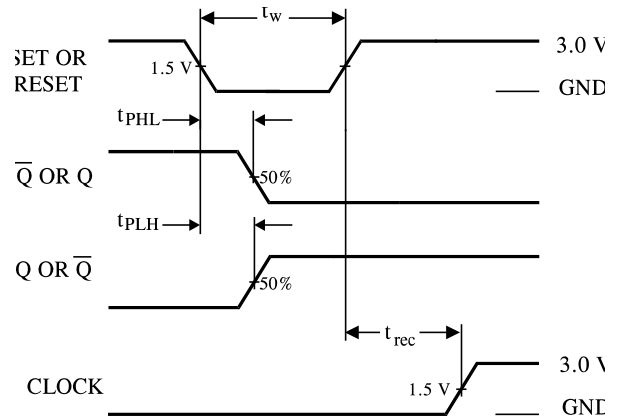
Figure 2. Switching Waveform
