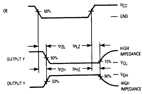
Figure 2. Switching Waveforms
