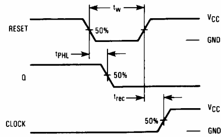
Figure 2. Switching Waveforms
