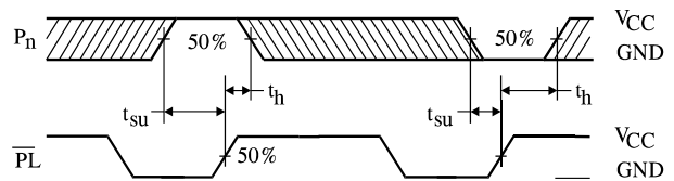
Figure 4. Switching Waveforms
