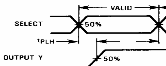
Figure 2. Switching Waveforms
