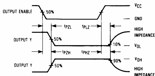
Figure 2. Switching Waveforms
