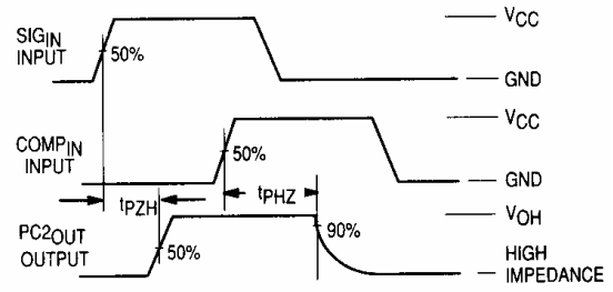
Figure 2. Switching Waveforms
