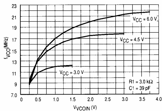
Figure 12A. VCO Frequency ( f_{VCO} ) as a Function of the VCO Input Voltage ( V_{COIN} )
