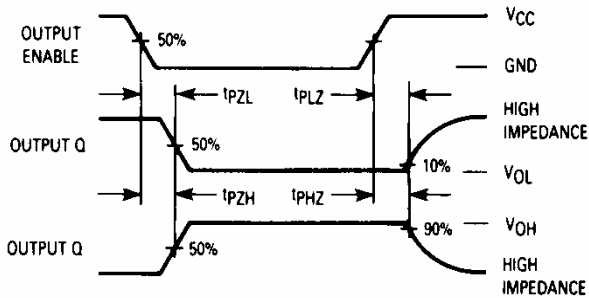
Figure 3. Switching Waveforms
