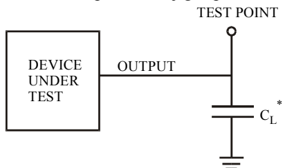
Figure 5. Test Circuit
