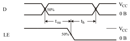
Figure 4. Switching Waveforms
