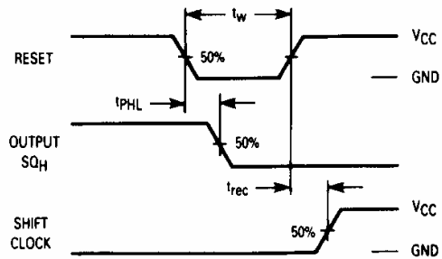
Figure 2. Switching Waveforms
