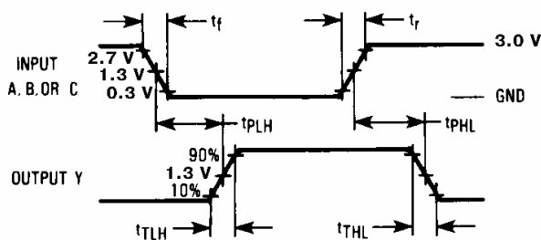
Figure 1. Switching Waveforms
