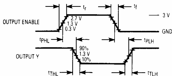
Figure 3. Switching Waveforms
