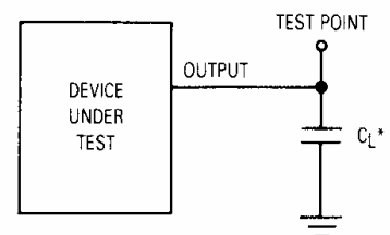
Figure 4. Test Circuit
