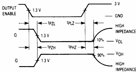
Figure 3. Switching Waveforms
