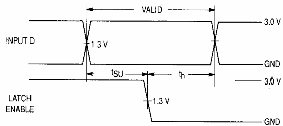
Figure 2. Switching Waveforms
