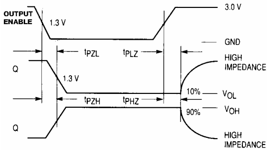
Figure 3. Switching Waveforms
