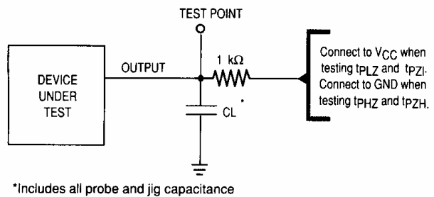
Figure 5. Test Circuit
