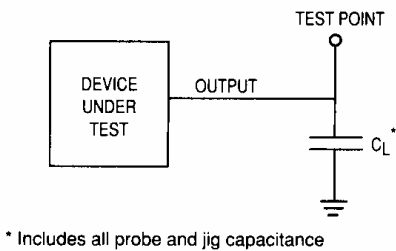
Figure 4. Test Circuit
