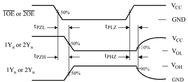
Figure 2. Switching Waveforms
