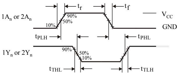
Figure 1. Switching Waveforms
