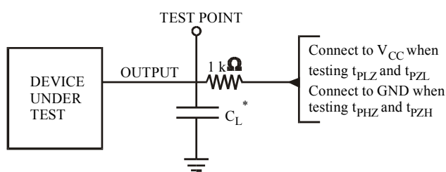
Figure 4. Test Circuit
