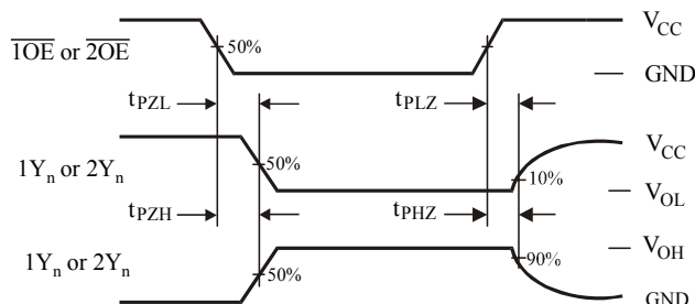
Figure 2. Switching Waveforms
