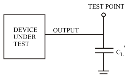
Figure 3. Test Circuit
