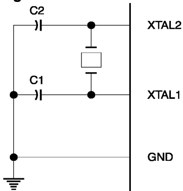
Figure 1. Oscillator Connections
