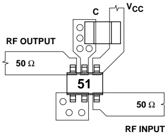
Figure 12. RF Layout.
