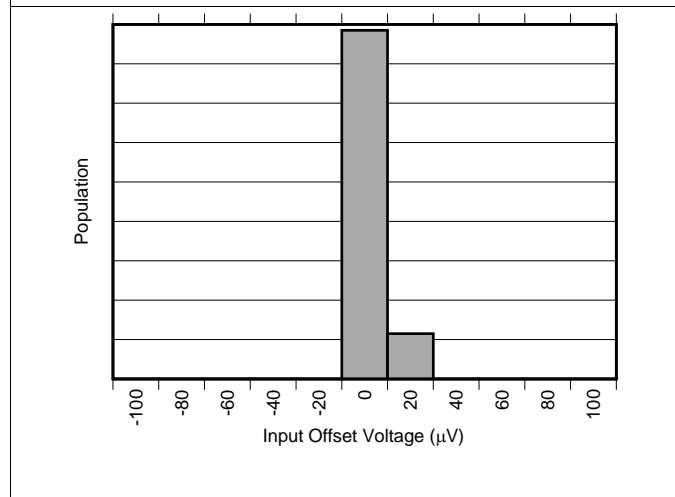
Figure 3. Input Offset Voltage Distribution (INA301A3-Q1)
