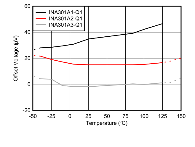
Figure 4. Input Offset Voltage vs Temperature
