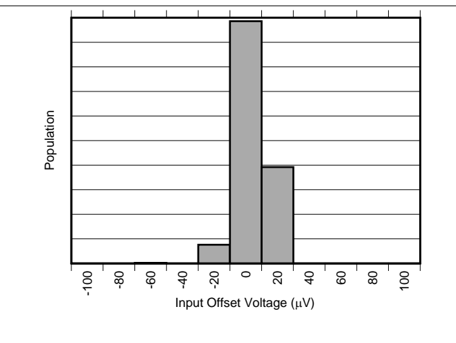
Figure 2. Input Offset Voltage Distribution (INA301A2-Q1)
