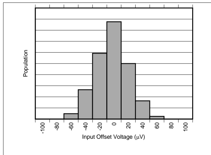
Figure 1. Input Offset Voltage Distribution (INA301A1-Q1)
