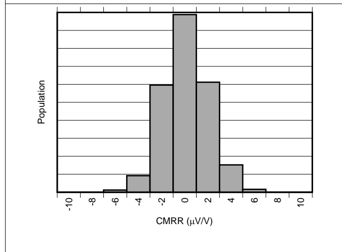
Figure 5. Common-Mode Rejection Ratio Distribution (INA301A1-Q1)
