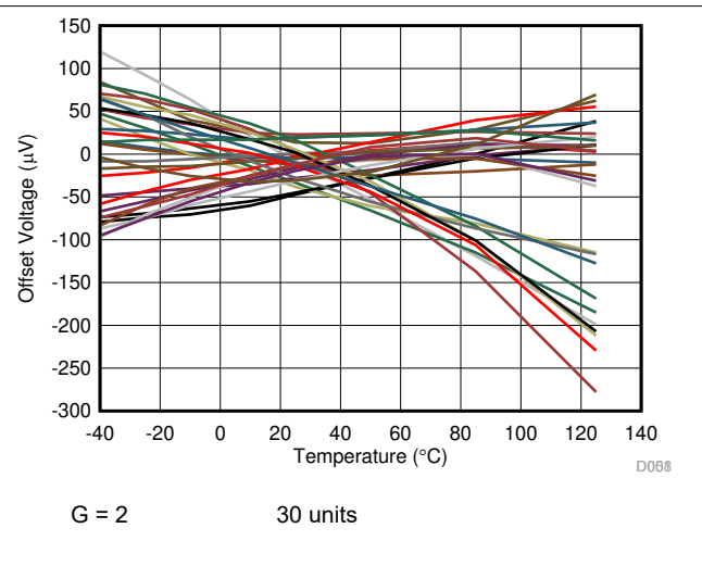
Figure 7-8. Output Offset Voltage vs Temperature
