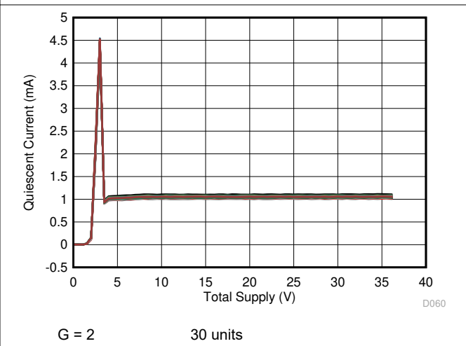
Figure 7-60. Supply Current vs Supply Voltage
