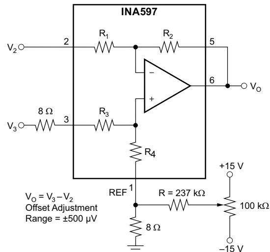
Figure 9-2. Offset Adjustment
