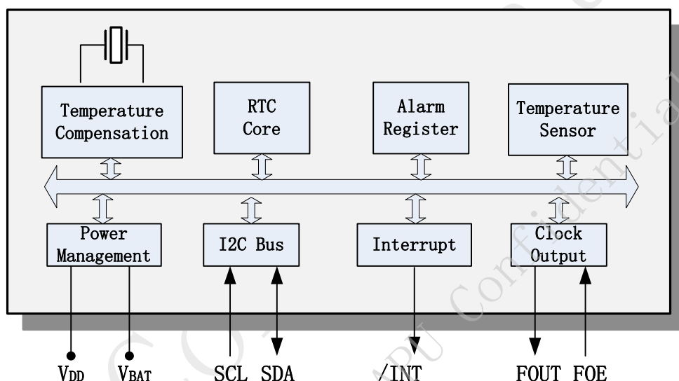
Figure 1. Block Diagram
