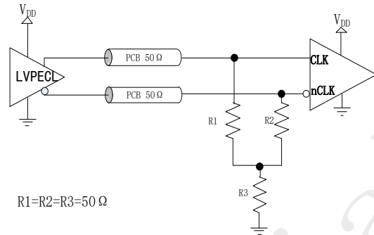
(b) LVPECL Input ("Y" Parallel Termination)
