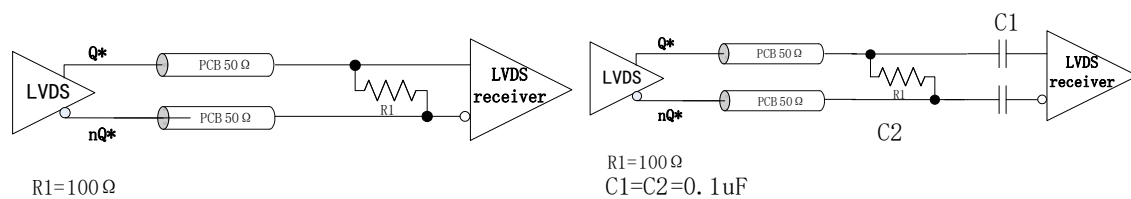
Figure 7. LVDS DC&amp;AC Coupling
