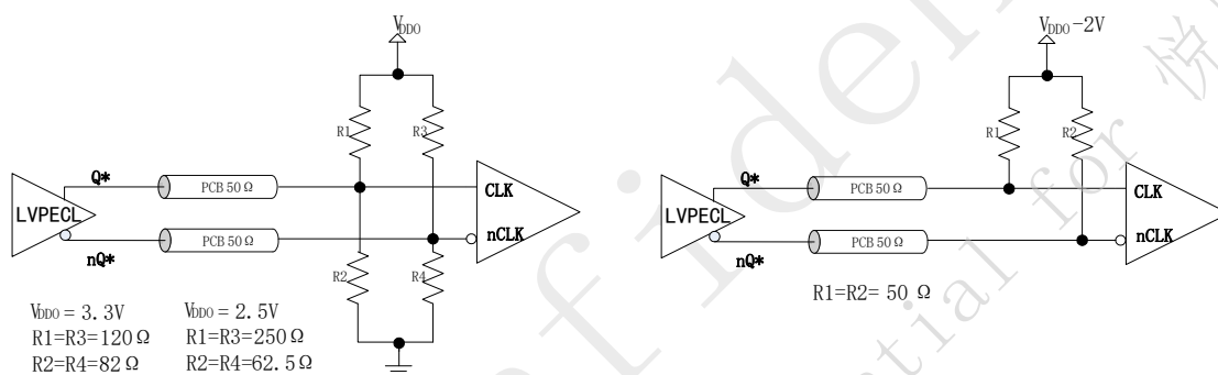
Figure 8. LVPECL DC Coupling
