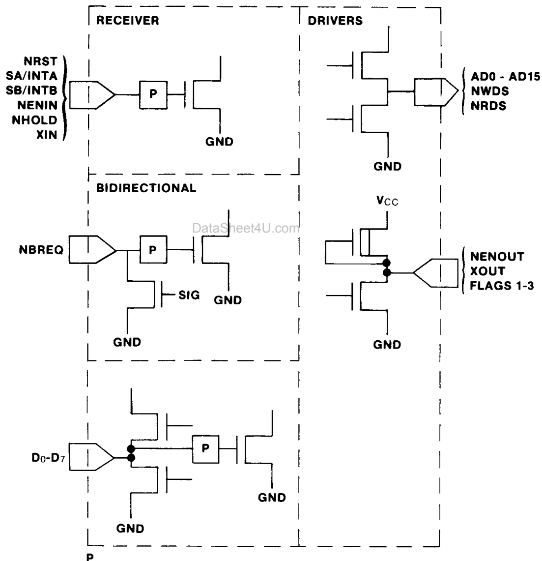
FIGURE 2. INS807X Drive and Receiver Equivalent Circuits
