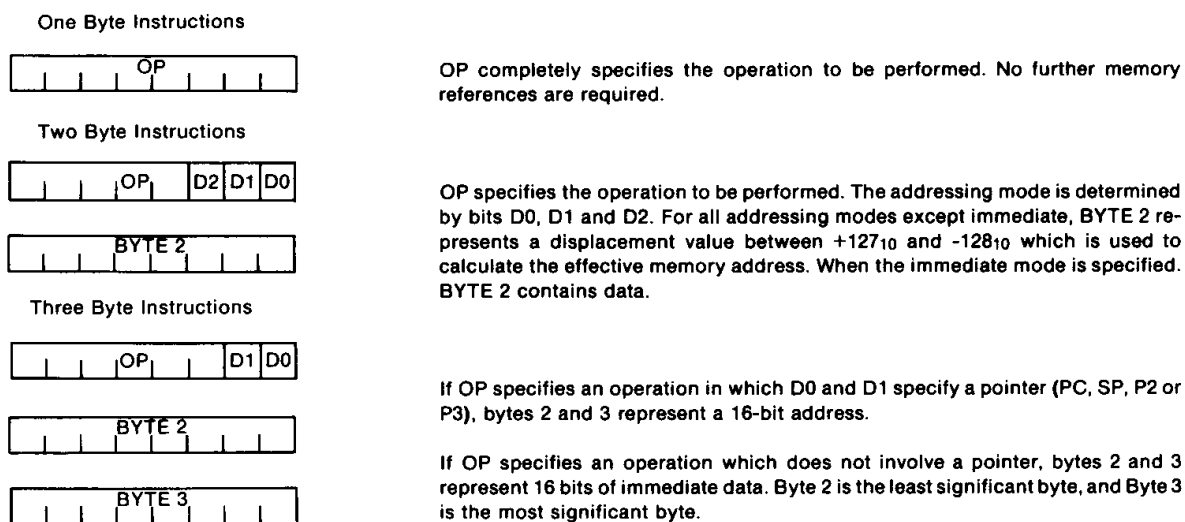
FIGURE 6. Instruction Byte Formats
