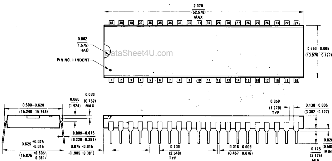
Plastic Dual In-Line Package (N) Order Number INS8070 or INS8072XXX/N
