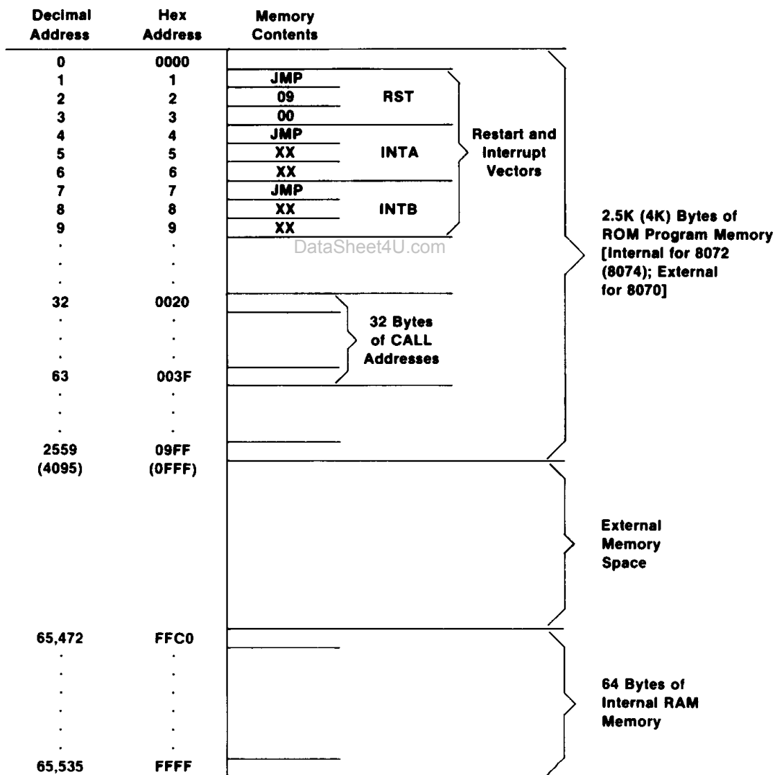
FIGURE 7. INS807X Memory Allocation
