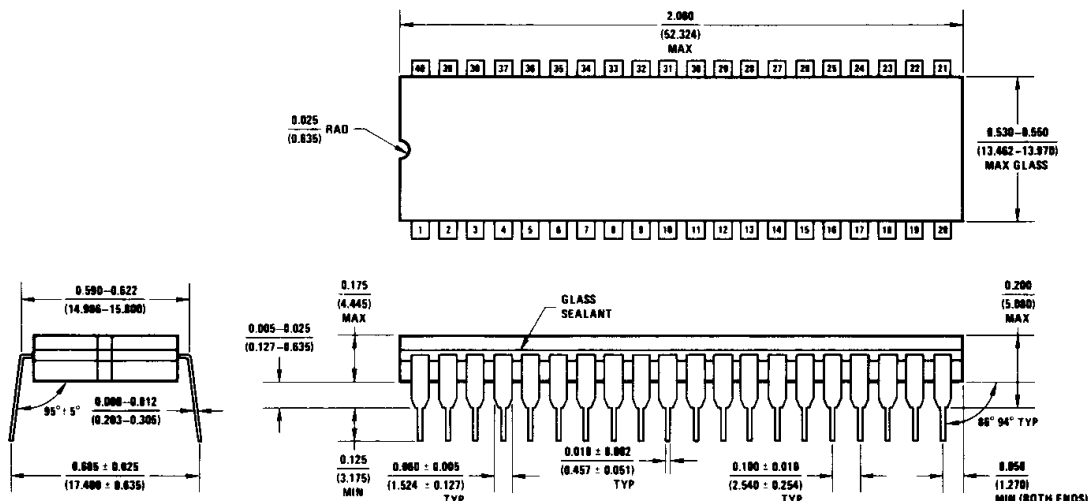
Ceramic Dual-In-Line Package [Cerdip (J)] Order Number INS8070J or INS8072XXX/J
