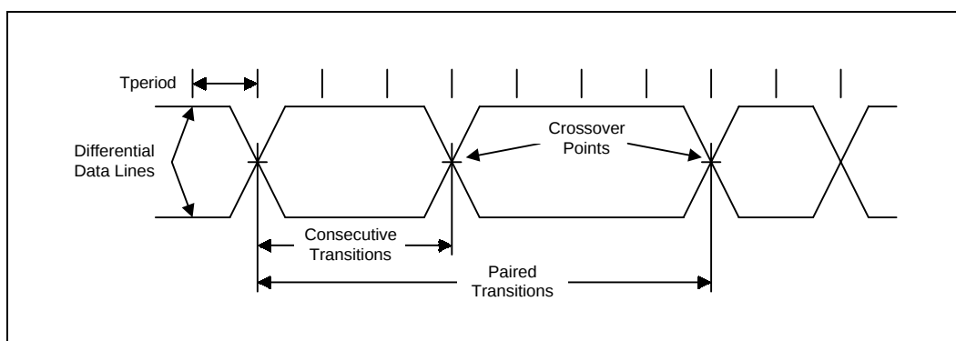
Figure 14-14. USB Jitter
