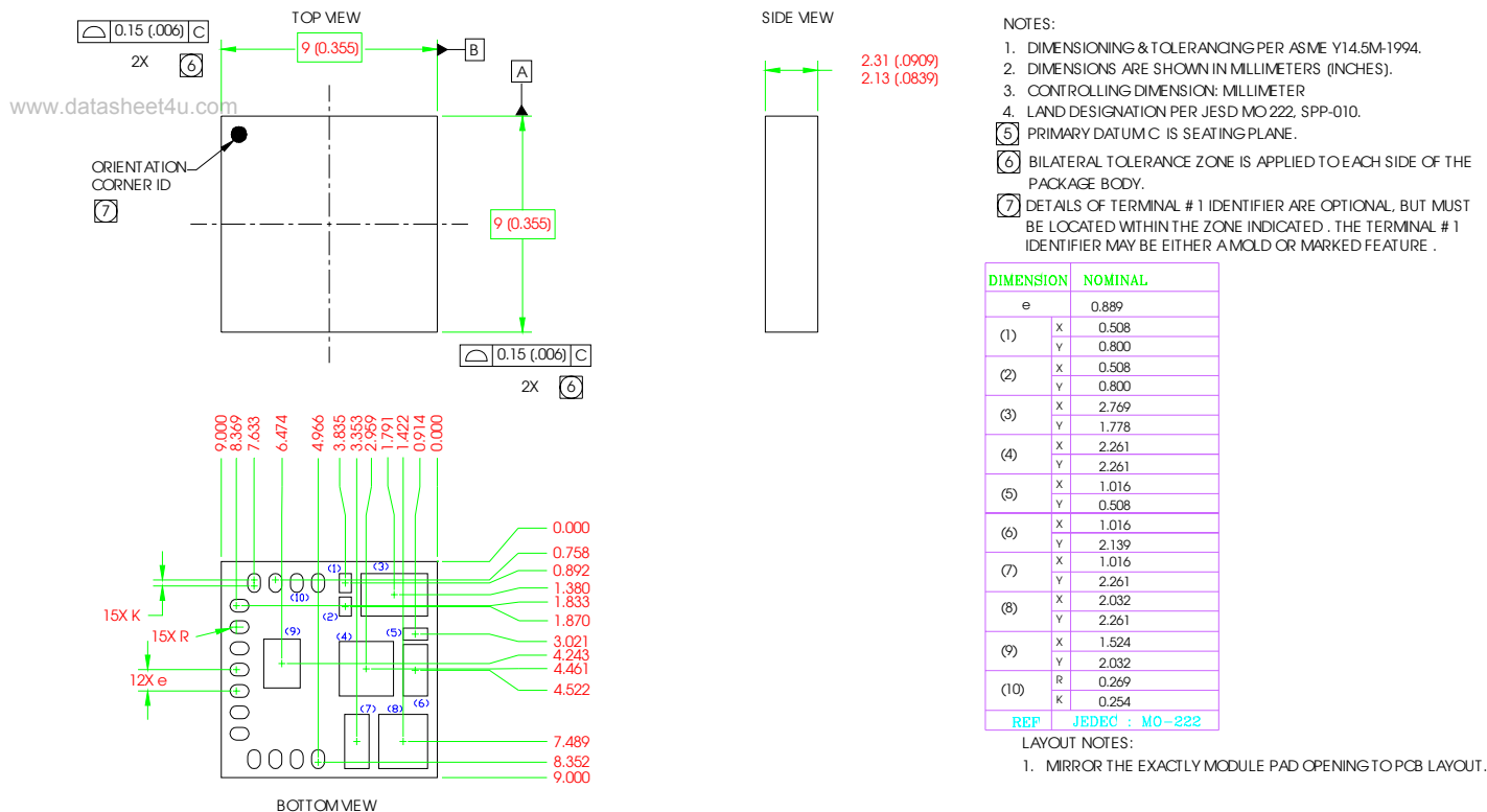
Fig. 25: Outline Drawing
