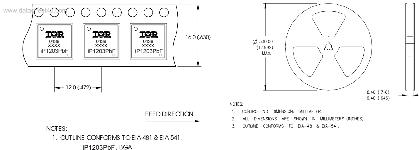
Fig. 26: Tape & Reel Information
