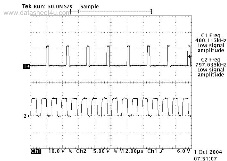
Ch1: Switching node, 400kHz Ch2: 800kHz external synchronization
