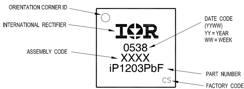
Fig. 27: Part Marking
