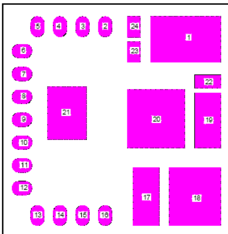
Fig. 22: iP1203PbF Pin Assignment
