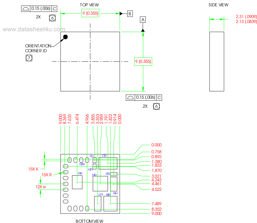
Fig. 25: Outline Drawing
