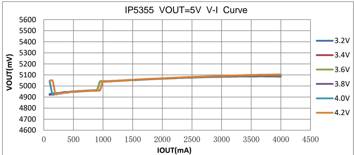
Figure 5 IP5355 VOUT=5V V-I Curve
