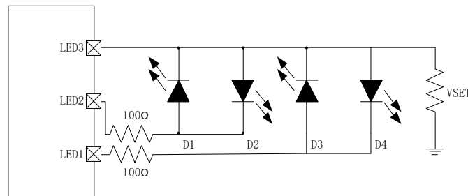
Figure 15 4LED circuits
